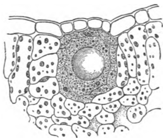
FIG 67. — A gland, in section, containing ethereal oil, in Dic-tamnus Frazinella ; much magnified. (From Sachs.)
